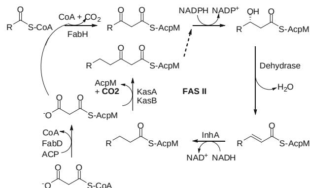
Scheme 1. General scheme of FAS-II system involved in mycolic acids biosynthesis.
