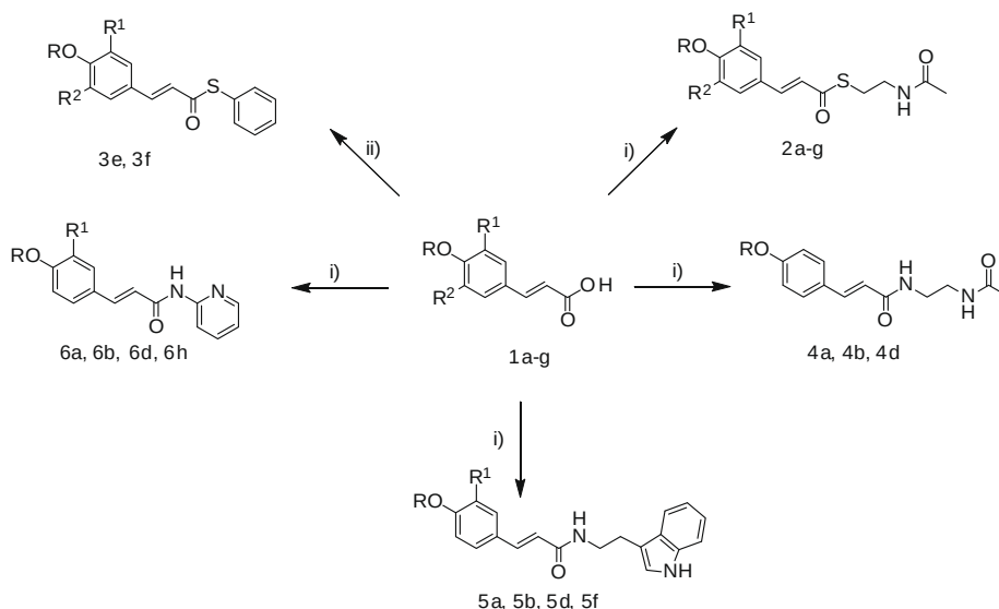
Scheme 2. Reagents and conditions: (i) DMAP, EDC, N -acetylcysteamine, 4-acetylenediamine, tryptamine, or 2-aminopyridine \text{CH}_2\text{Cl}_2 , rt, 24 h; (ii) (\text{COCl})_2 , DMF, \text{CH}_2\text{Cl}_2 , 0 °C, 1 h, then thiophenol, BuLi, THF, –30 °C, 2 h.
